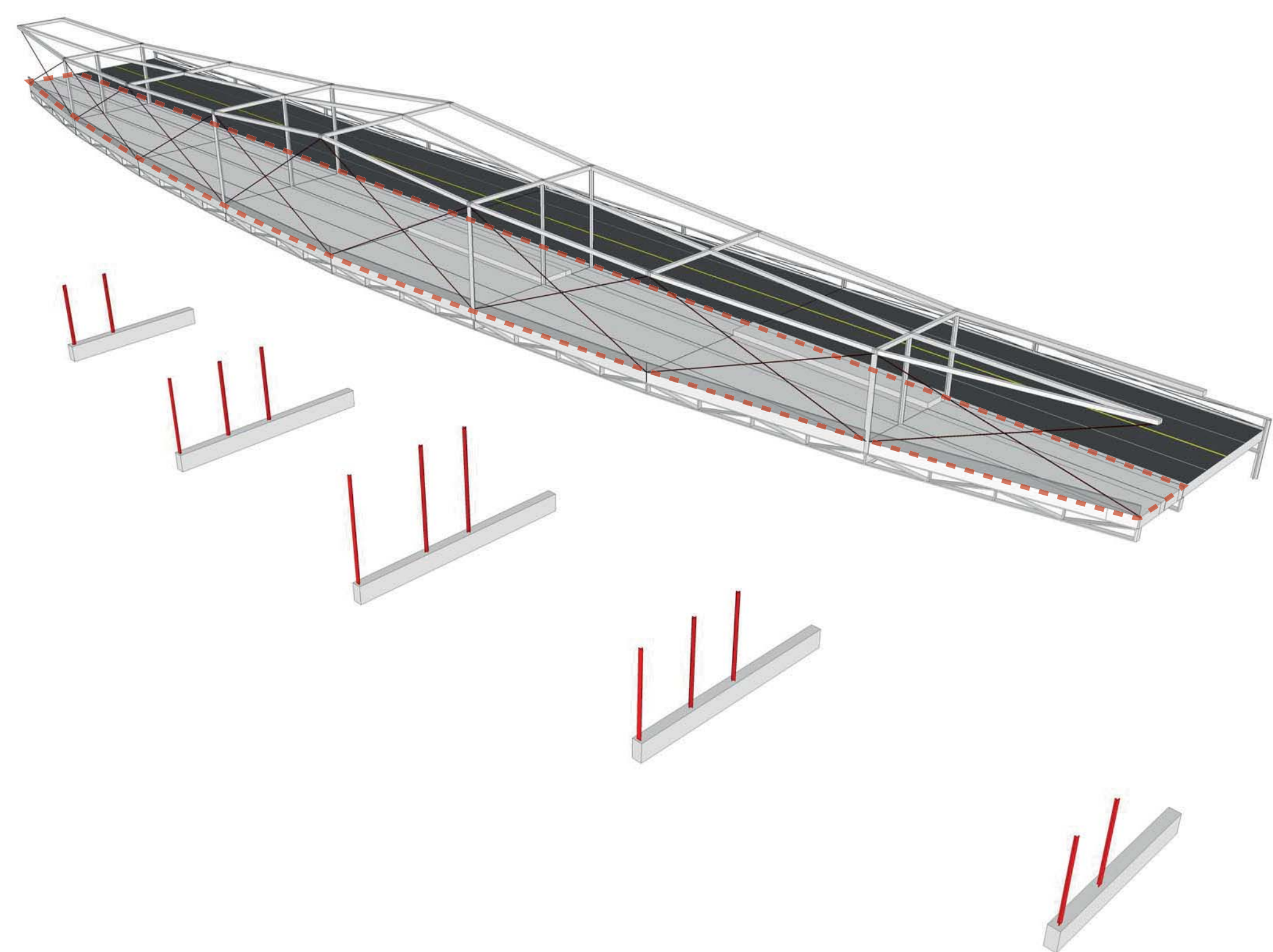
PARTITIONS CAN CHANGE ELEVATION WITH HYDRAULIC LIFT TECHNOLOGY
