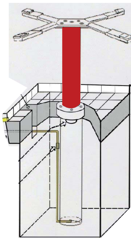
PARTITIONS CAN CHANGE ELEVATION WITH HYDRAULIC LIFT TECHNOLOGY
